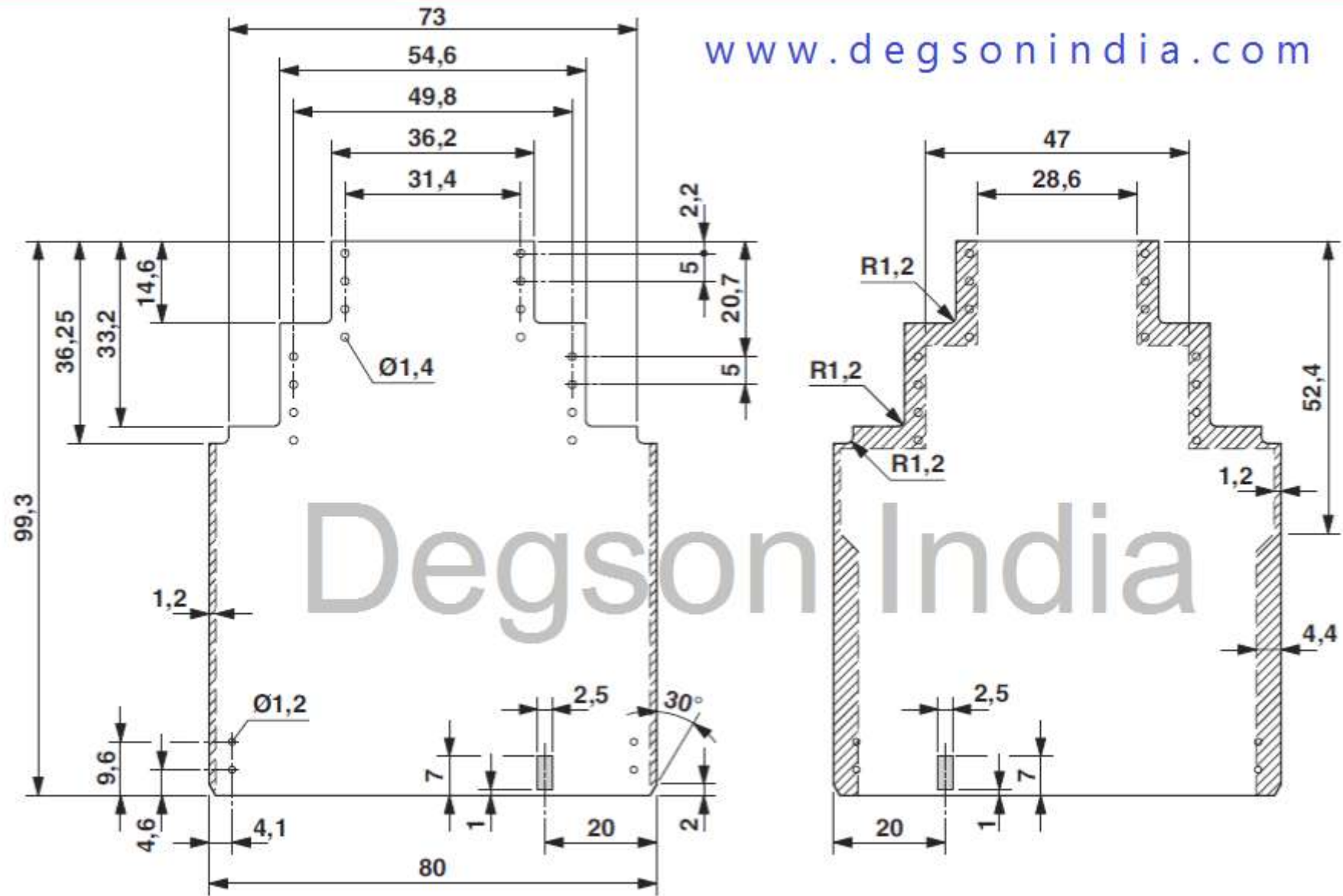
PCB Drawing of FMET-04P-14-15AH (All Dimensions are in mm)
