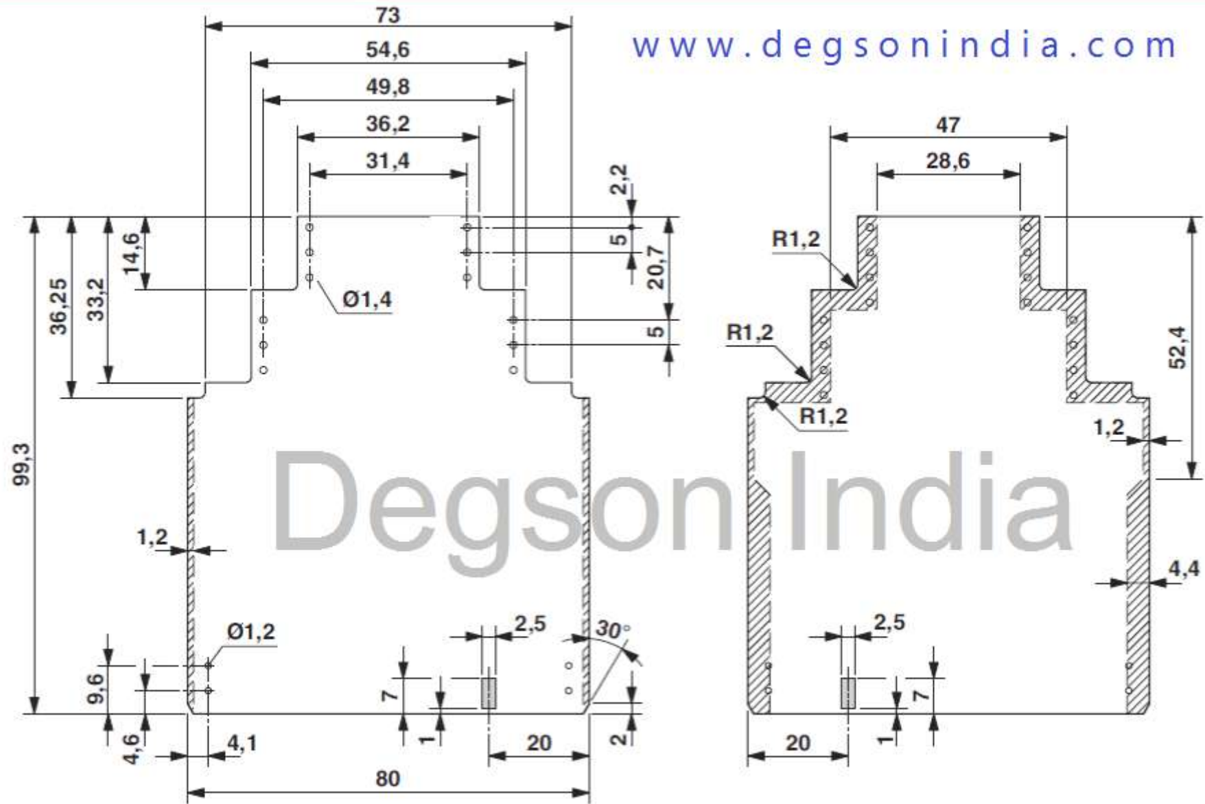
PCB Drawing of FMET-06P-14-15AH (All Dimensions are in mm)
