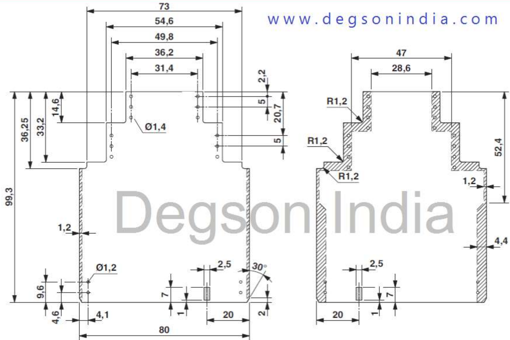
PCB Drawing of FMET-03P-14-15AH (All Dimensions are in mm)
