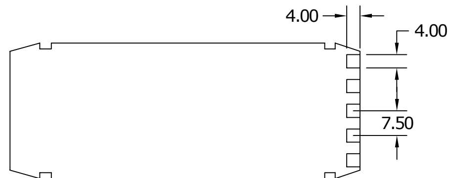
Main PCB with 16 pole terminal pads
