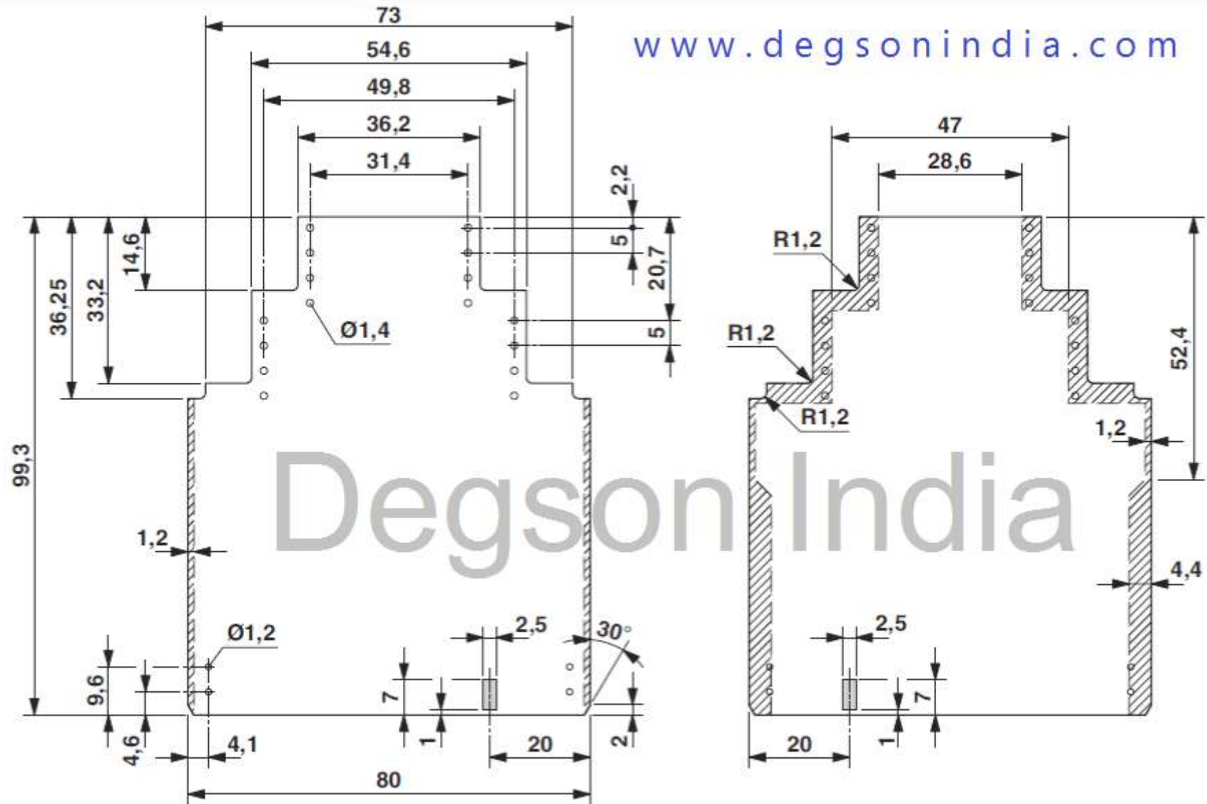
PCB Drawing of FMET-08P-14-15AH (All Dimensions are in mm)
