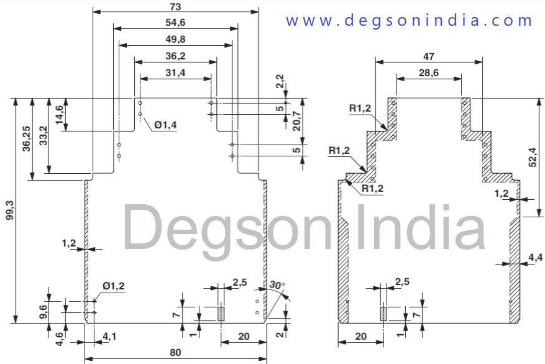
PCB Drawing of FMET-02P-14-05AH (All Dimensions are in mm)
