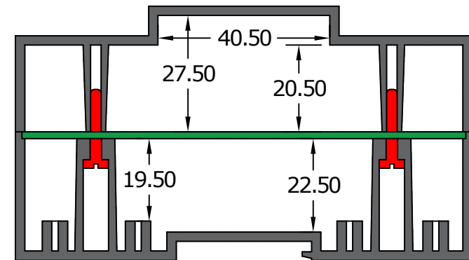
Slice View
