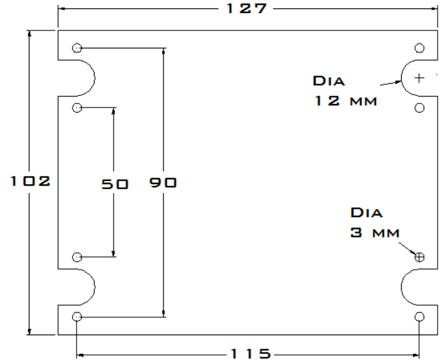
DRAWING OF BOTTOM PCB
