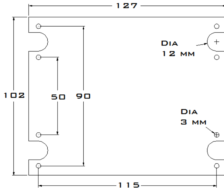
DRAWING OF BOTTOM PCB
