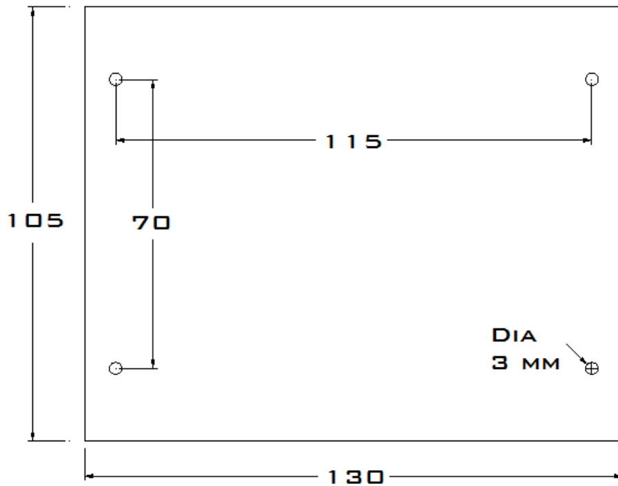
DRAWING OF TOP PCB
