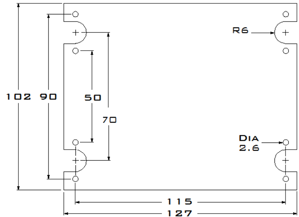
DRAWING OF BOTTOM PCB
