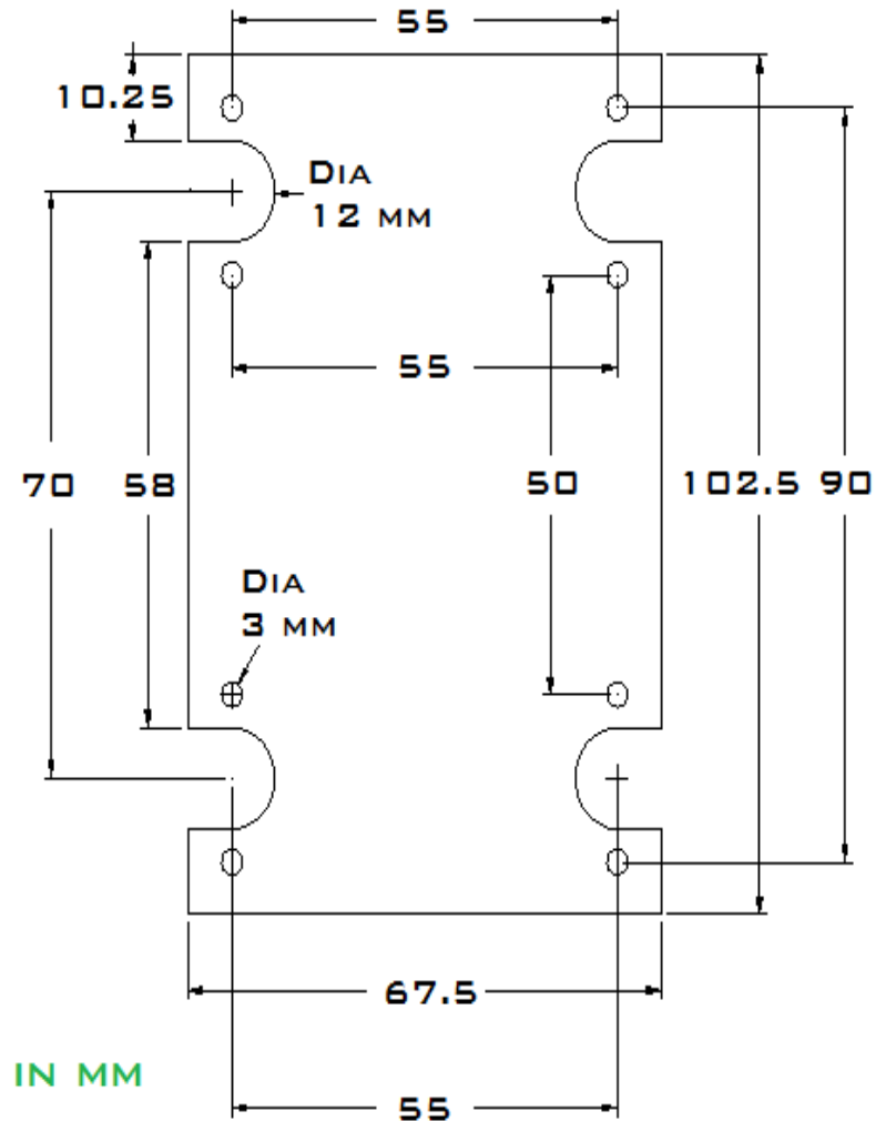
DRAWING OF BOTTOM PCB
