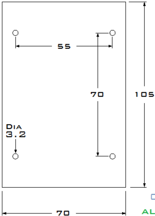
DRAWING OF TOP PCB
