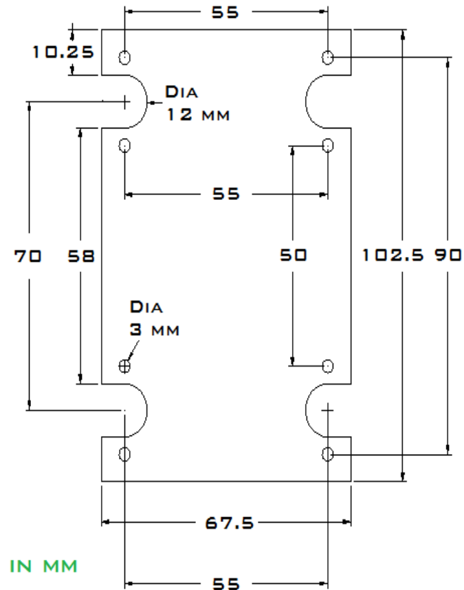
DRAWING OF BOTTOM PCB
