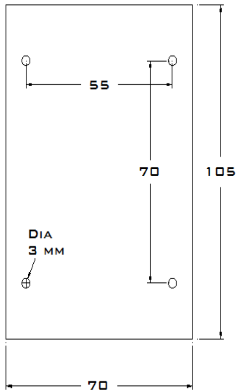
DRAWING OF TOP PCB
