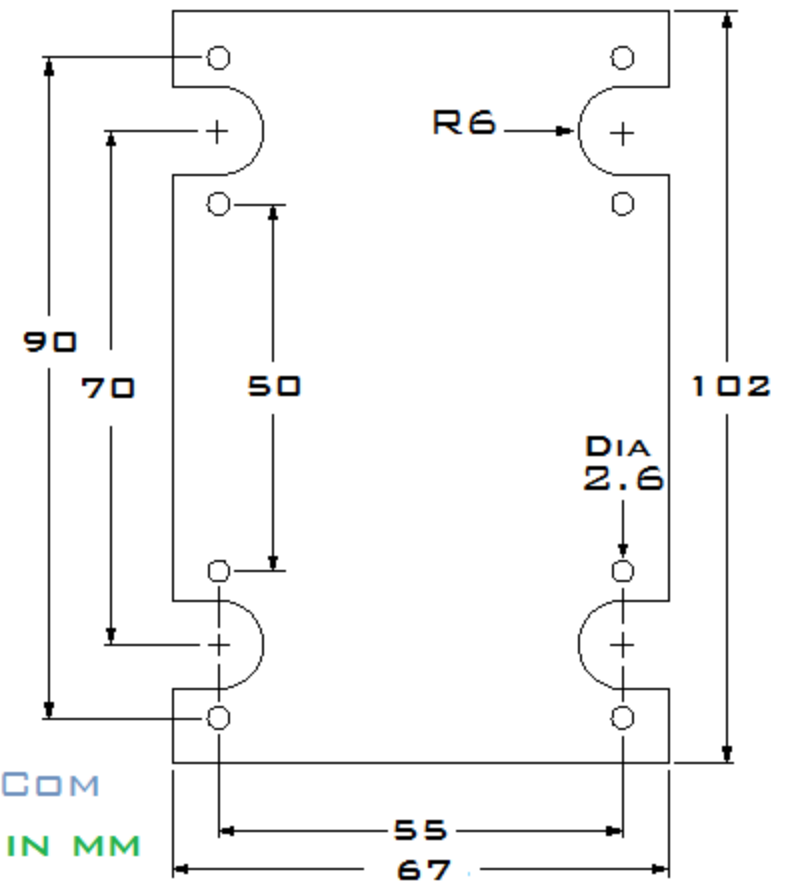
DRAWING OF BOTTOM PCB
