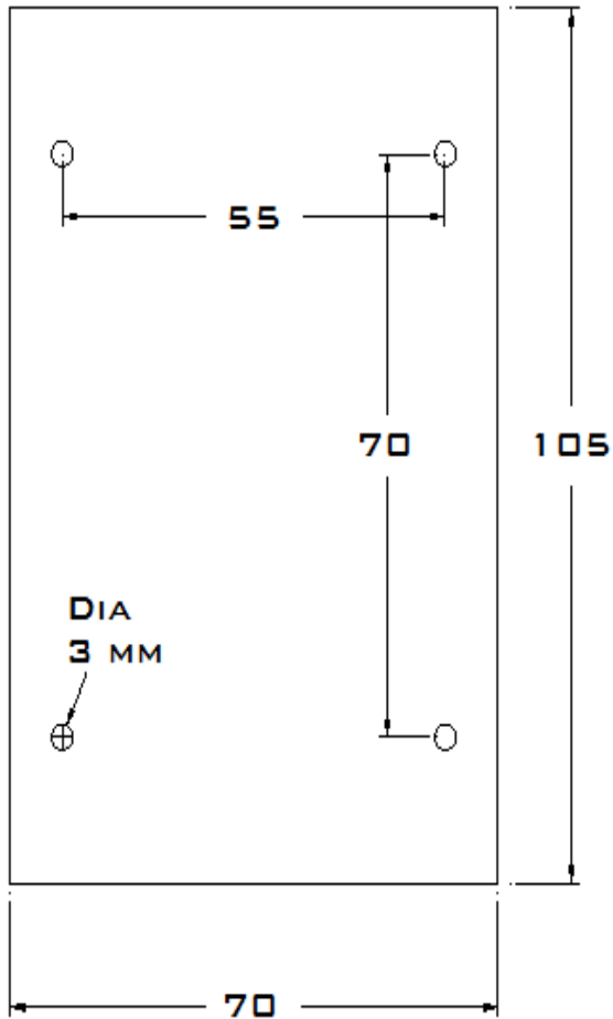
DRAWING OF TOP PCB
