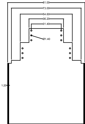
Horizontal Dimensions
